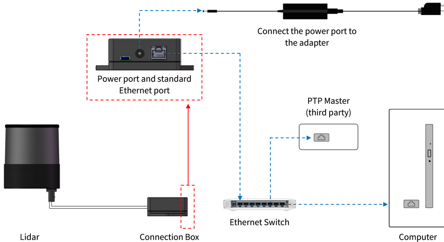
Figure 20. Connection with PTP (hardware device)
